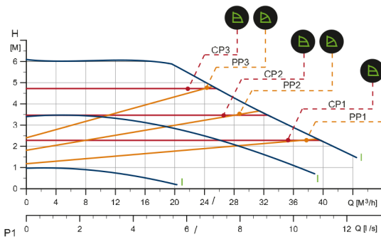
MAGNA 1 80-60 F 1 x 230 V, 50/60 Hz PN 6 Kod :99221406
